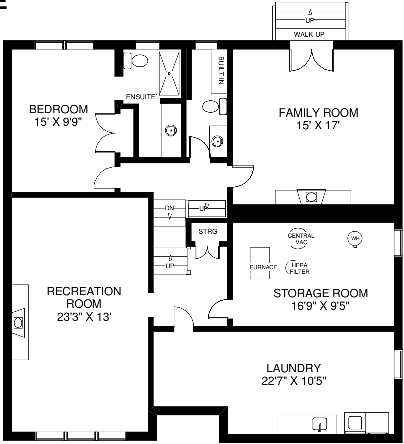
GROUND FLOOR APPROXIMATELY 720 SQ FT LOWER FLOOR APPROXIMATELY 930 SQ FT
