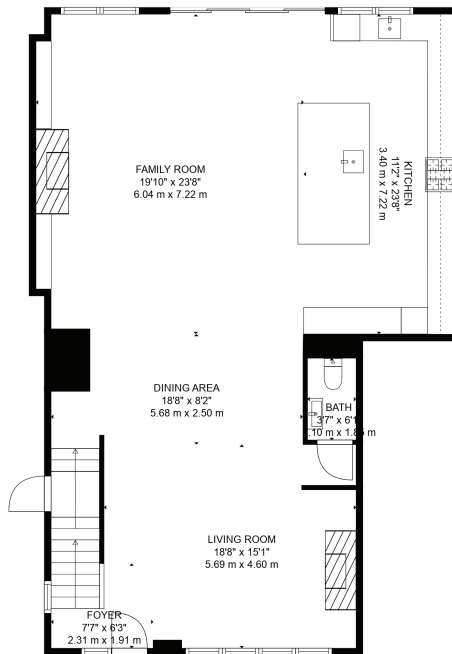
FLOOR 2
