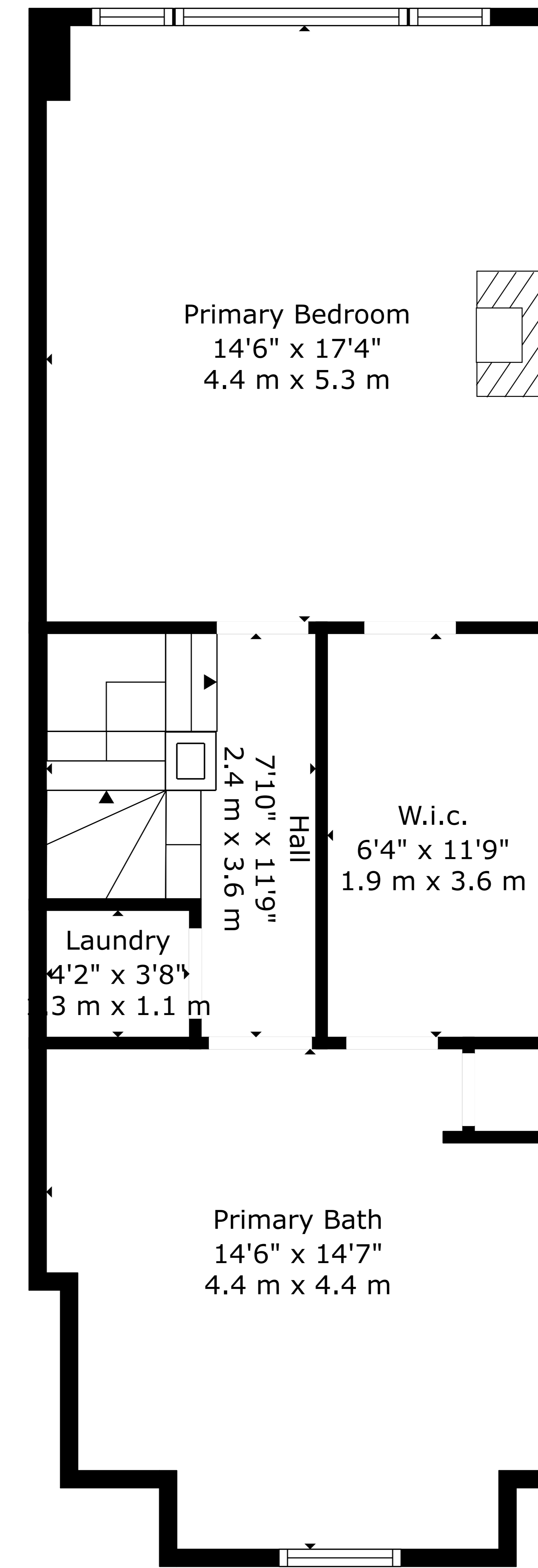
Floor 4
