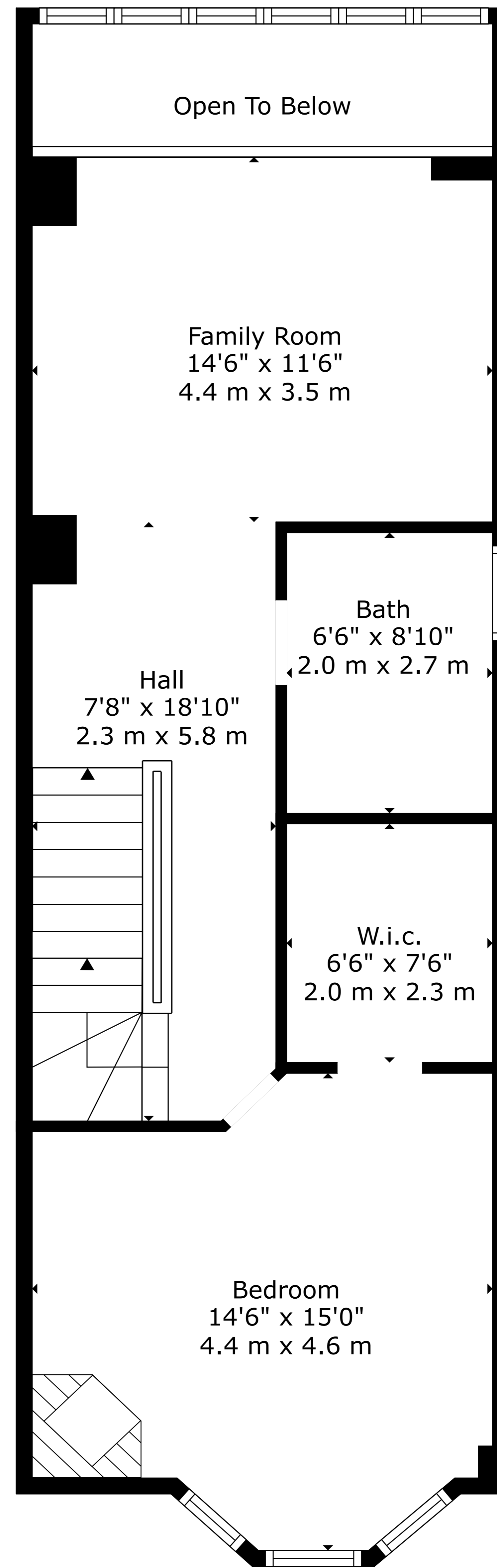
Floor 3
