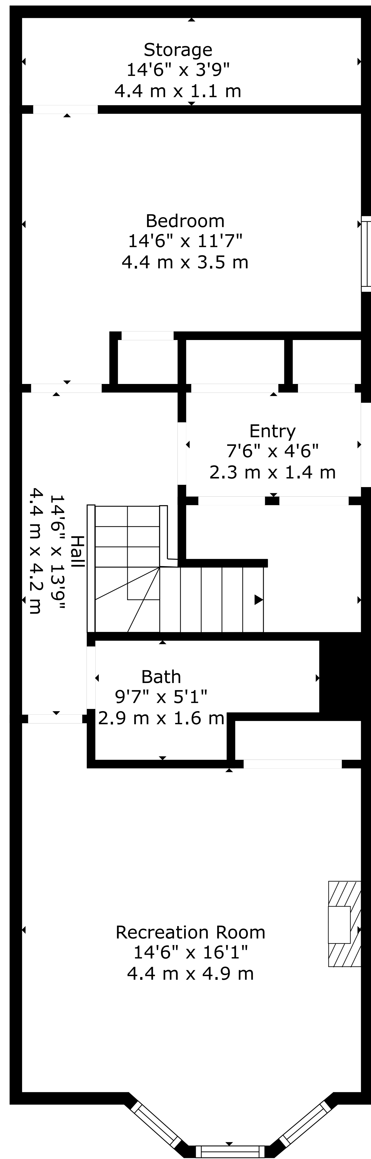
Floor 1
