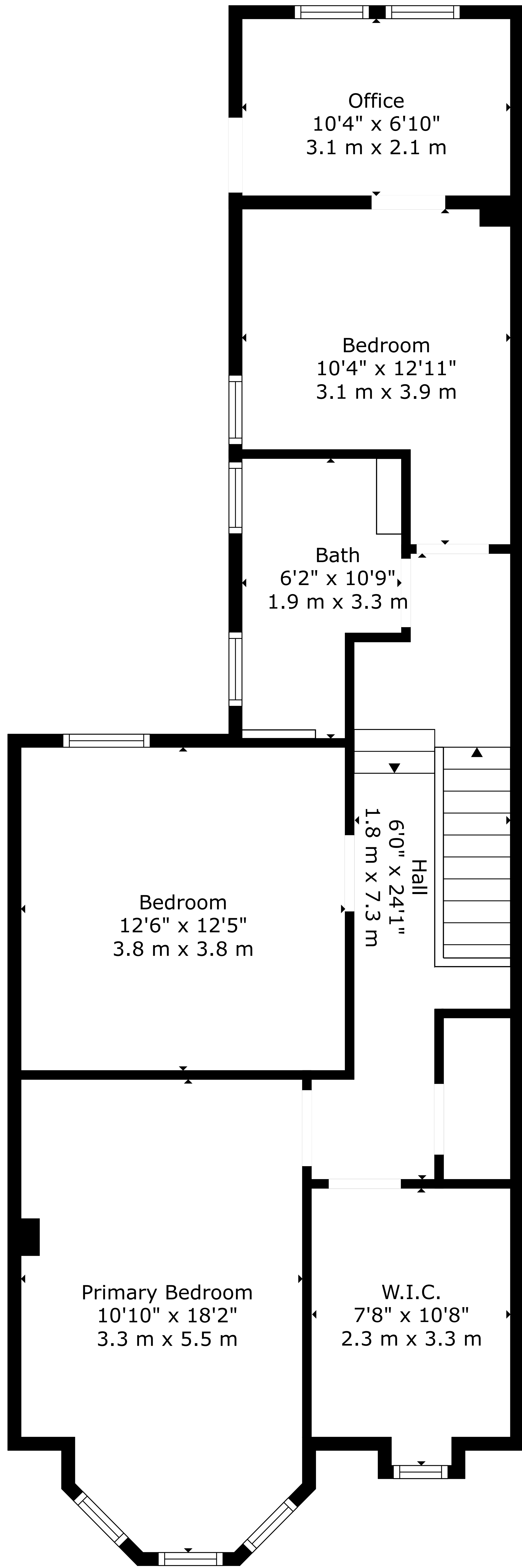
Floor 3
